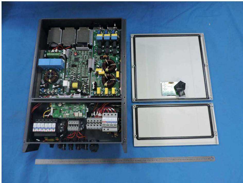
Internal view-1
